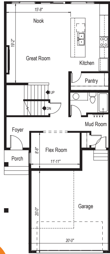
Main Floor Full Bathroom (md24b)
