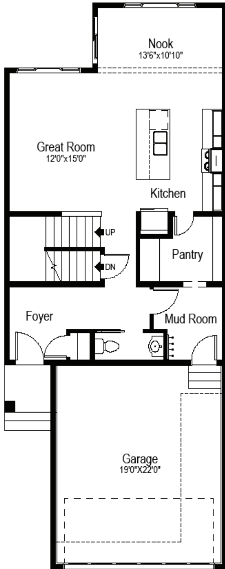
MAIN FLOOR - 870 SQ.FT.
