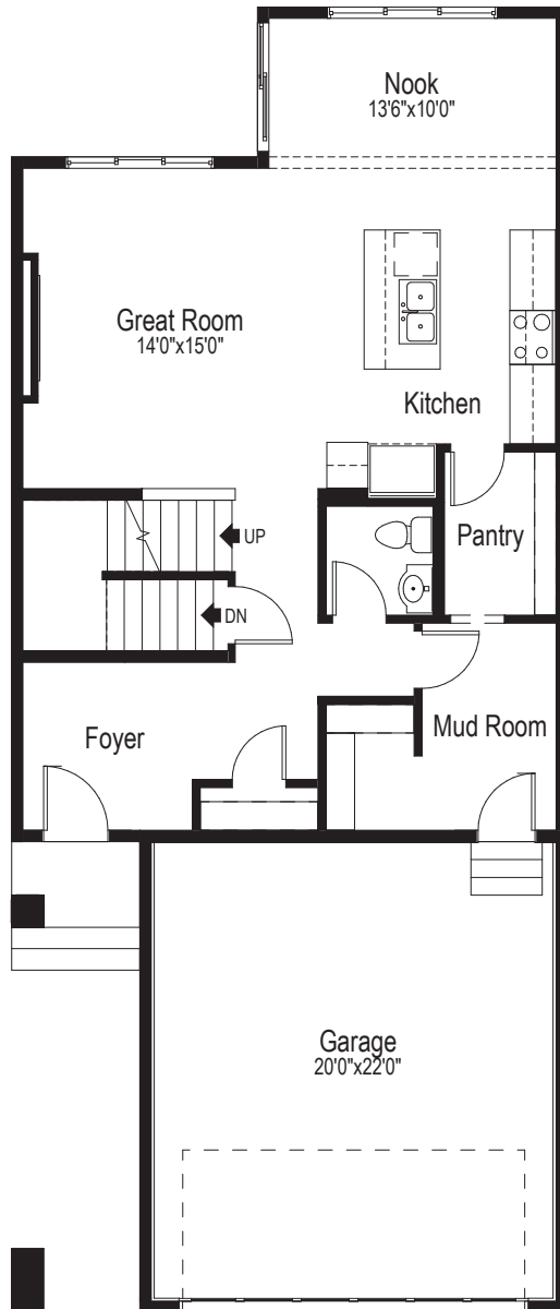
MAIN FLOOR - 934 SQ.FT.
